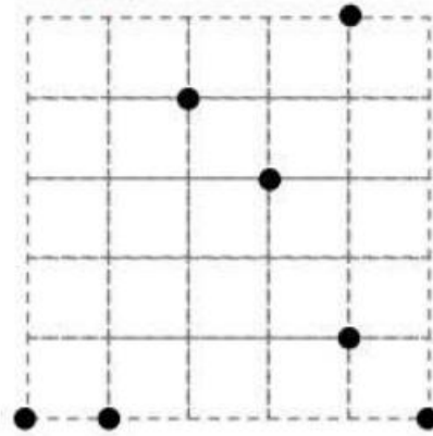
Triangle rectangle
