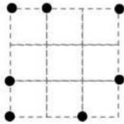
Rectangle
