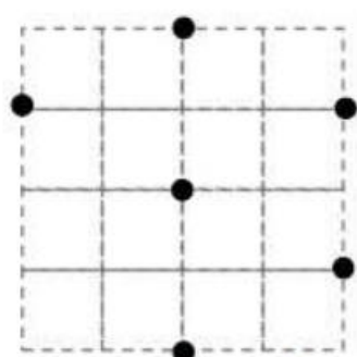
Triangle rectangle
