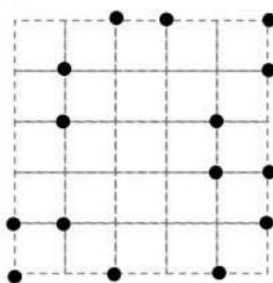
Rectangle
