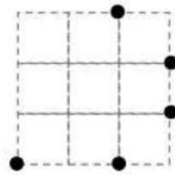
Triangle rectangle
